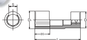
Socket for Lambda Probes Open section allows for use with wire/connector.
